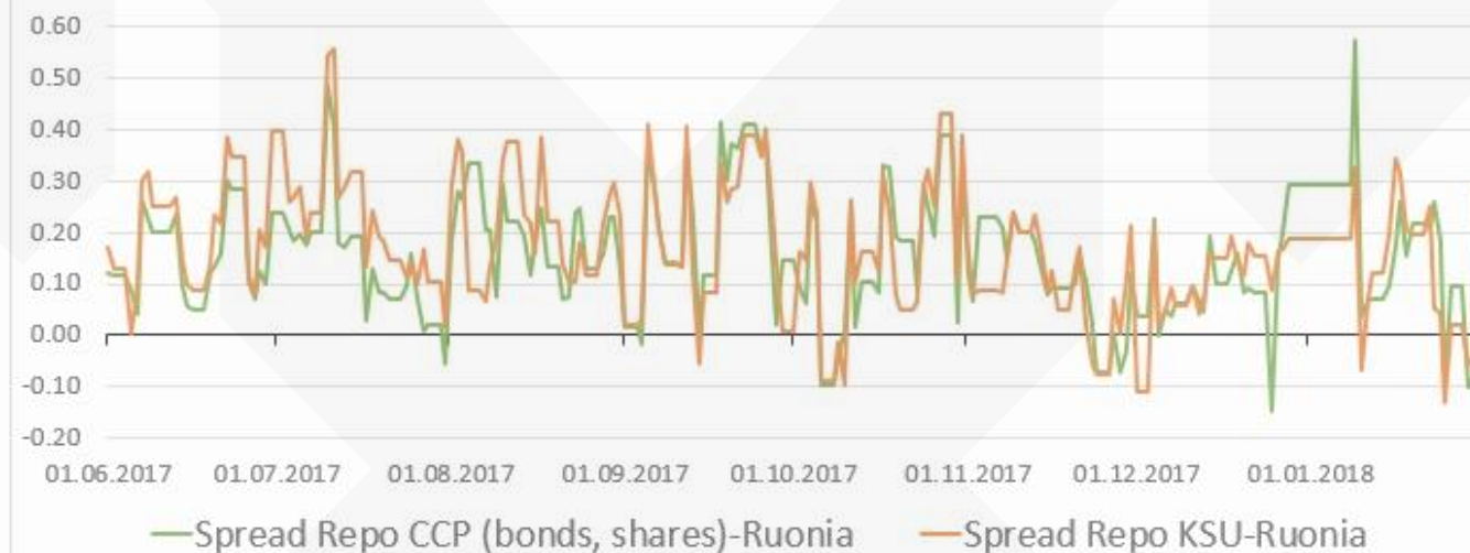
Spreads Repo - RUONIA
